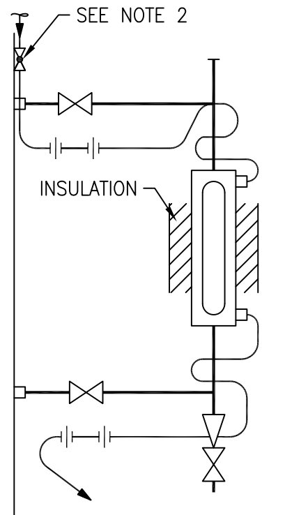
DETAIL 'B' DETAIL FOR INTEGRAL JACKETED GAUGE GLASS
